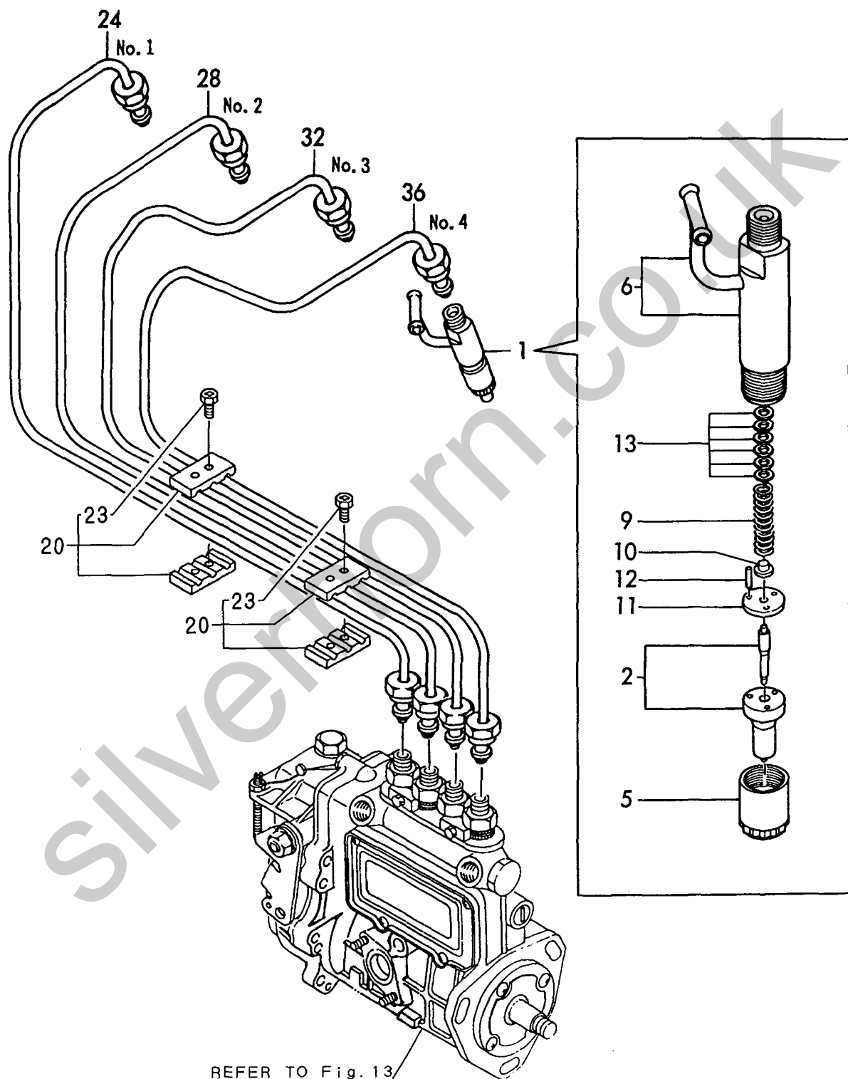
Fig. 14 FUEL INJECTION PIPE
