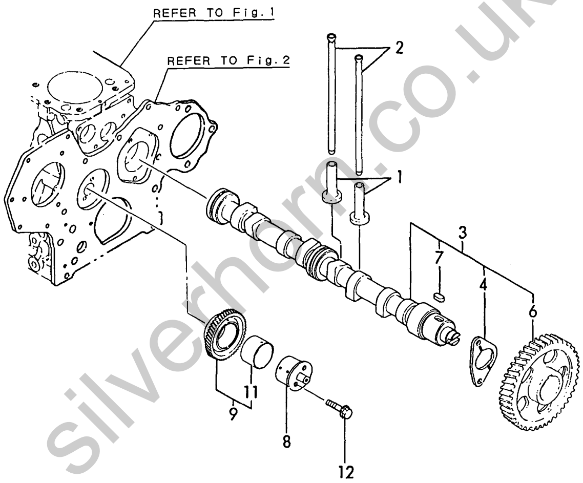
Fig. 7 CAMSHAFT & DRIVING GEAR
