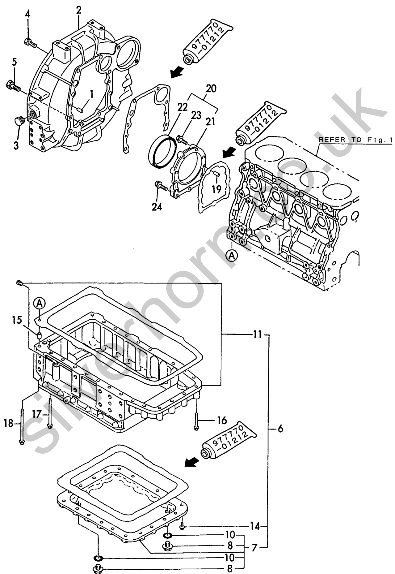
Fig. 3 FLYWHEEL HOUSING & LUB. OIL SUMP
