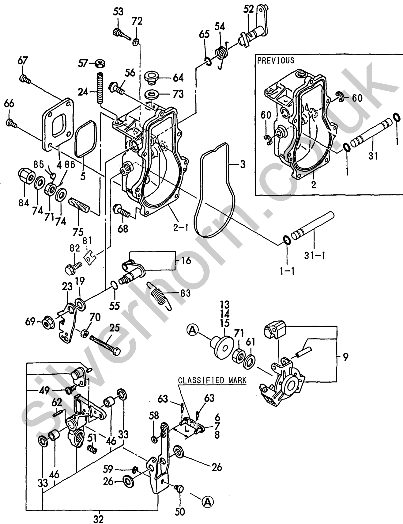
Fig. 16 GOVERNOR
