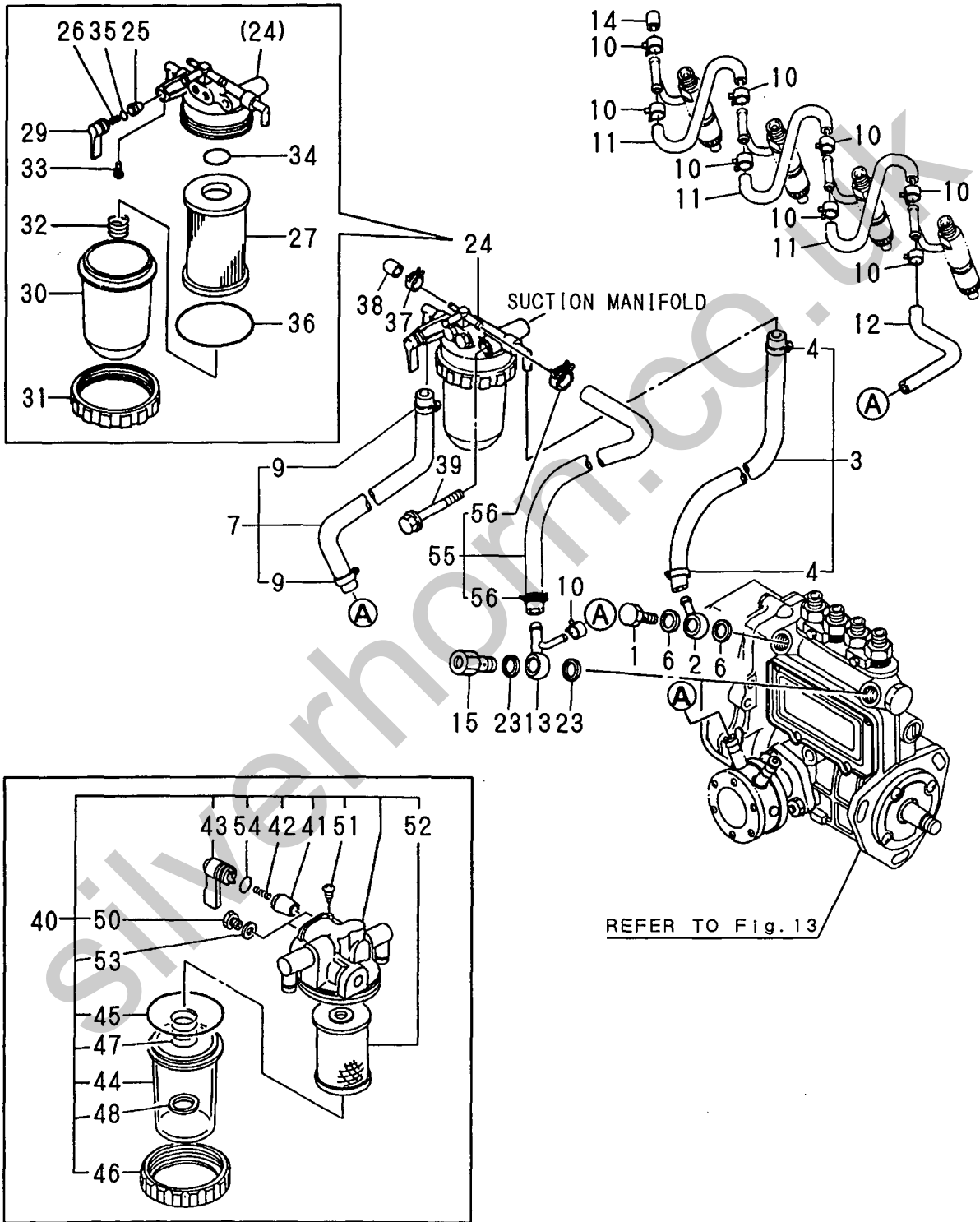
Fig. 15 FUEL PIPE
