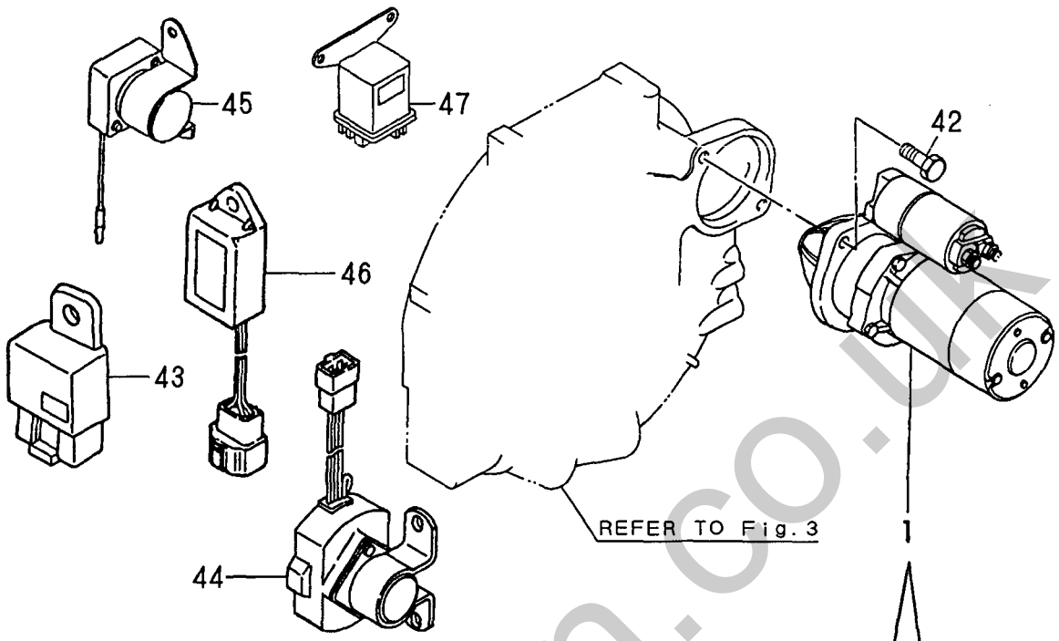
Fig. 17 STARTING MOTOR
