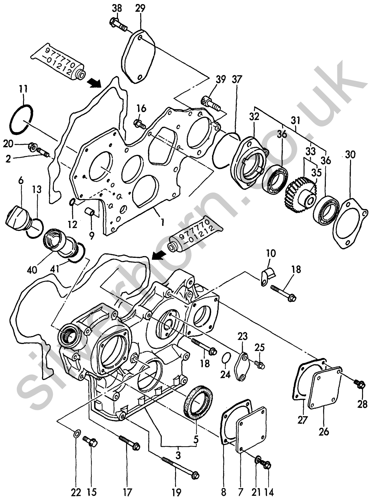
Fig. 2 GEAR HOUSING
