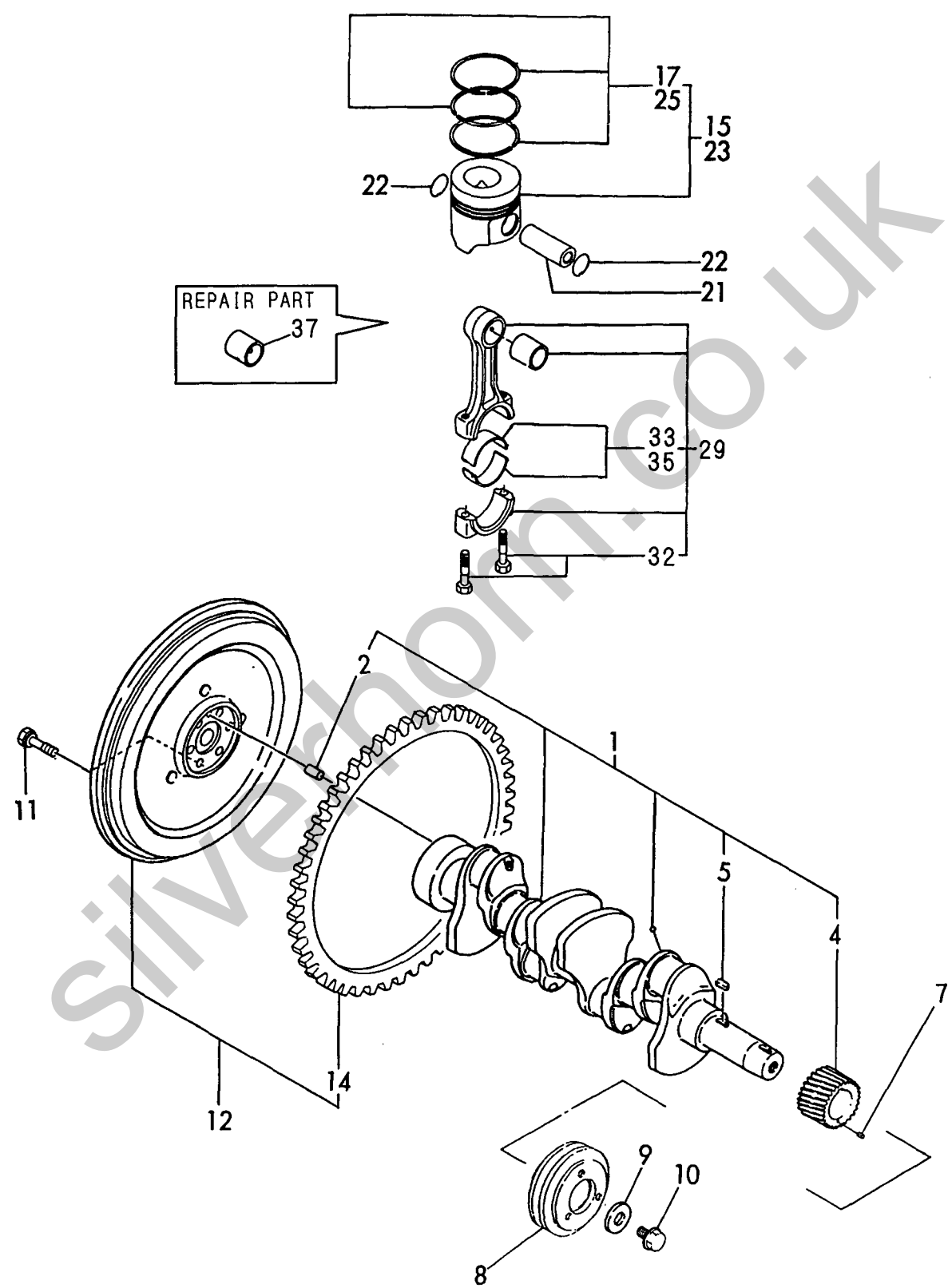
Fig. 9 CRANKSHAFT & PISTON
