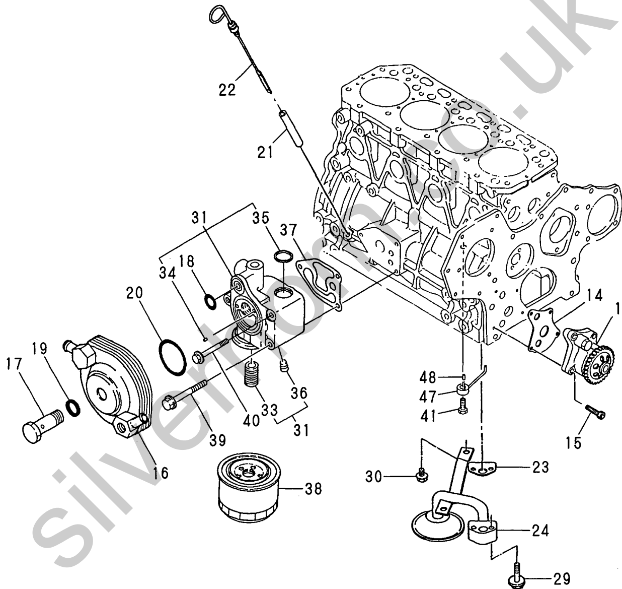
Fig. 10 LUB. OIL SYSTEM
