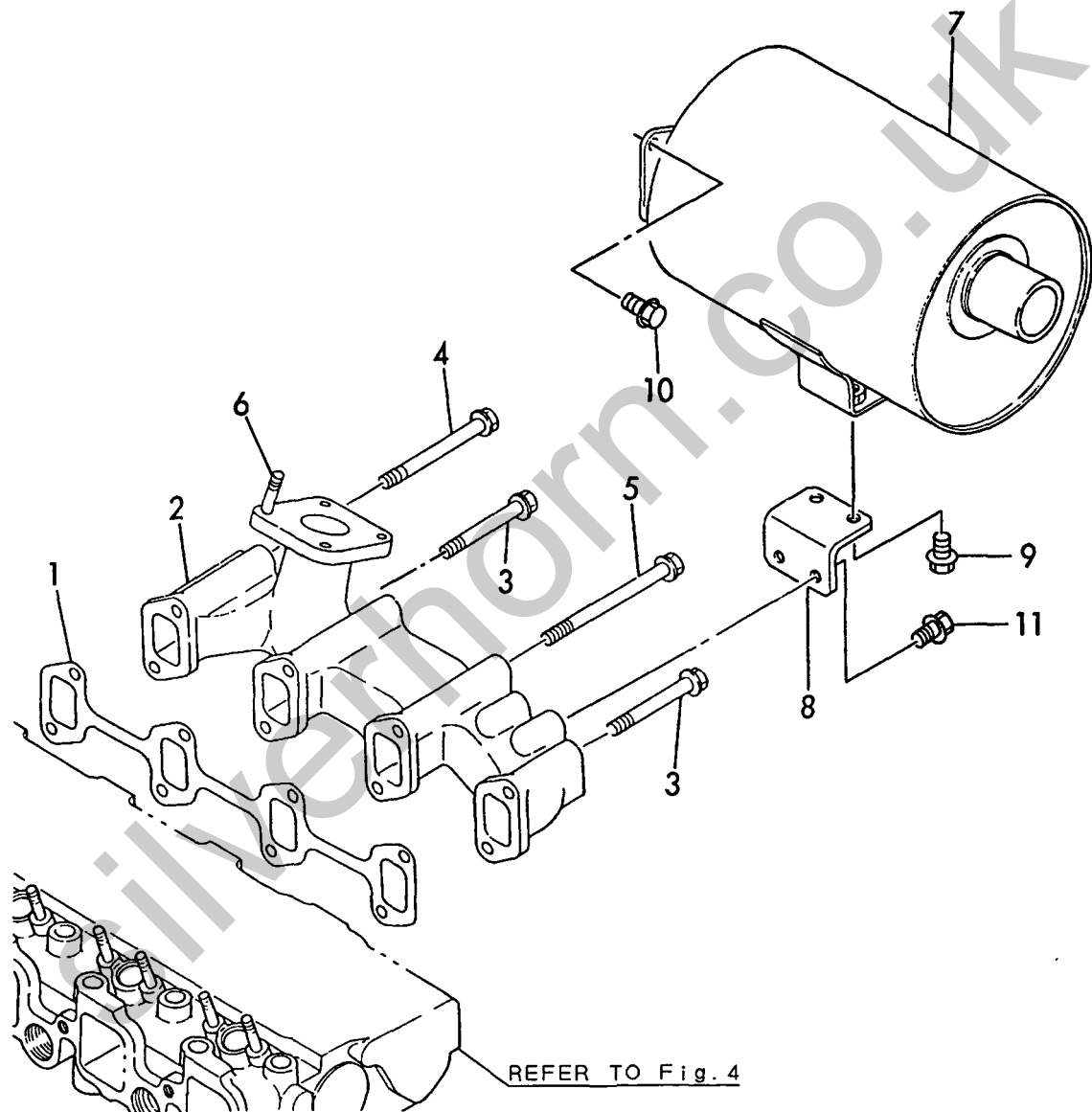
Fig. 6 EXH. MANIFOLD & SILENCER
