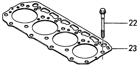
Fig. 1 CYLINDER BLOCK
